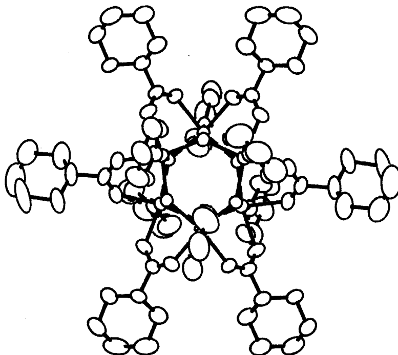
FIGURE 2 ORTEP plot of [\text{PhSn}(\text{O})\text{O}_2\text{CC}_6\text{H}_{11}]_6 viewed down the S_6 axis with thermal ellipsoids at the 50% probability level
